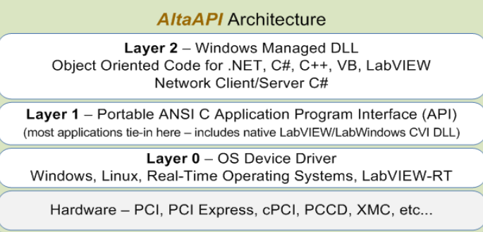
Alta's Advanced Software Architecture
