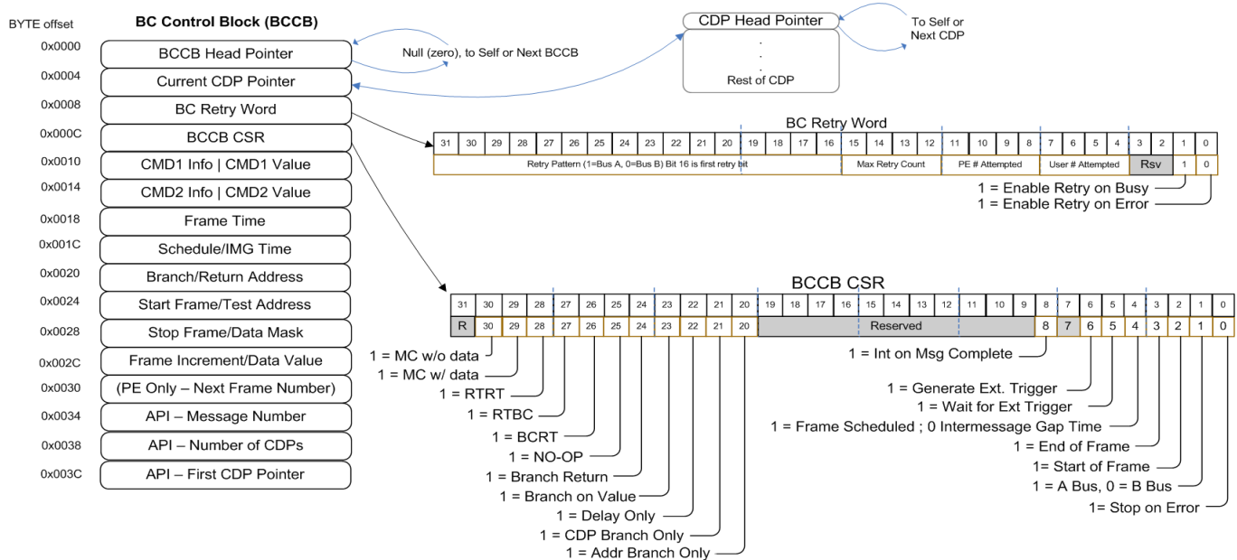
Figure BC-2: BCCB Data Structure
