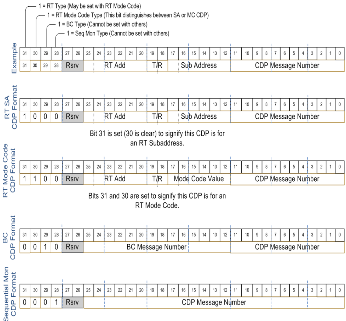
CDP/Interrupt API Info Word Format
