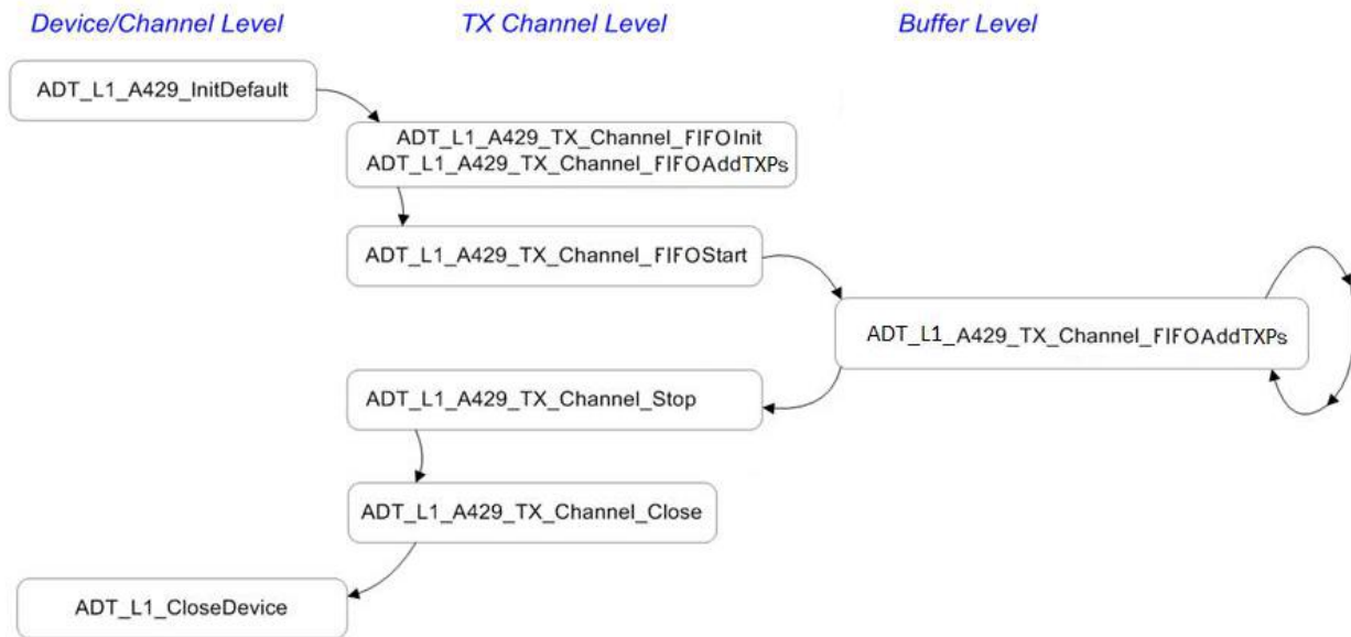
Figure ARINC-TX : Basic TX FIFO API Flow
