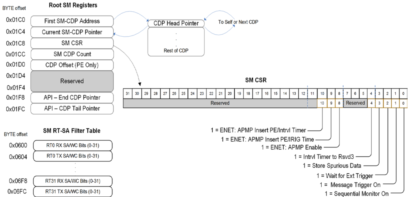
Figure SM-1: Root and Extended SM Data Structures
