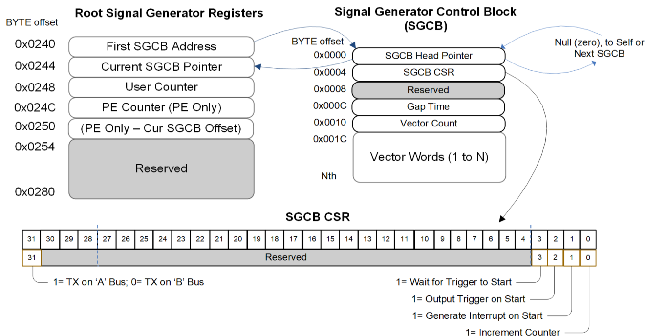
Figure SG-1: Signal Generator Data Structures
